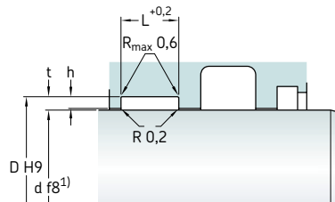
Rod application (dynamic on the inside surface)
