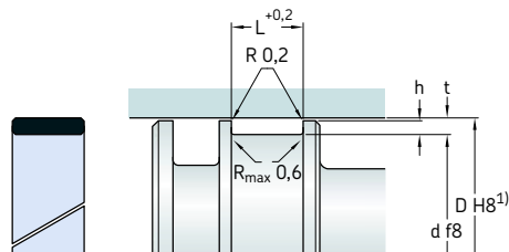
Piston application (dynamic on the outside surface)
